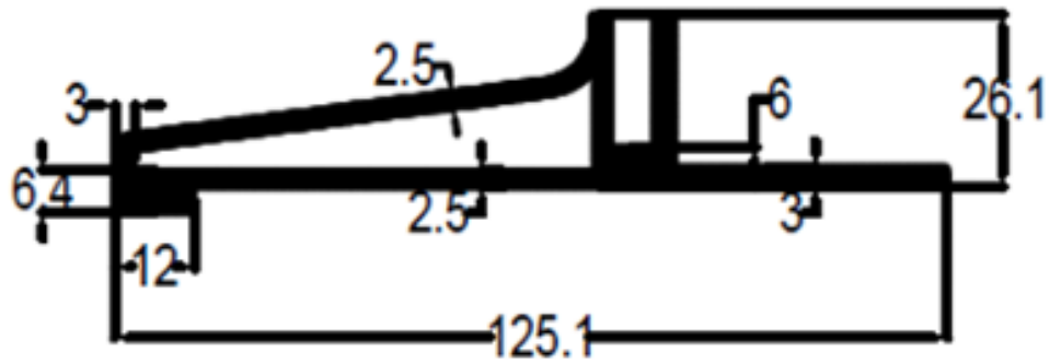
Section No :MCO637(SECTION 5 INCH) 6900GM / 12 FT
