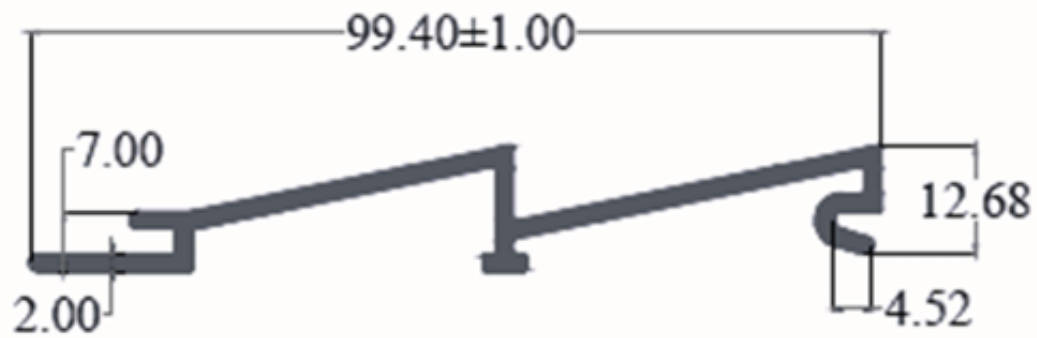
Section No : MCO632 (2 HUT OPEN ) 2750GM / 12 FT
