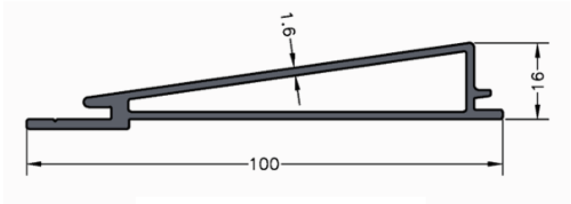
Section No: MCO629(TRIANGLE 4 INCH) 3500GM / 12 FT
