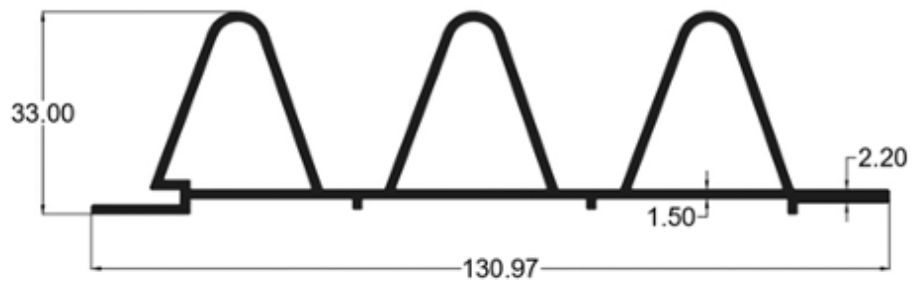
Section No: MCO626(3 CONE CLOSE) 5150GM / 12 FT
