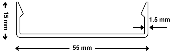
Cover Plate(101022)
