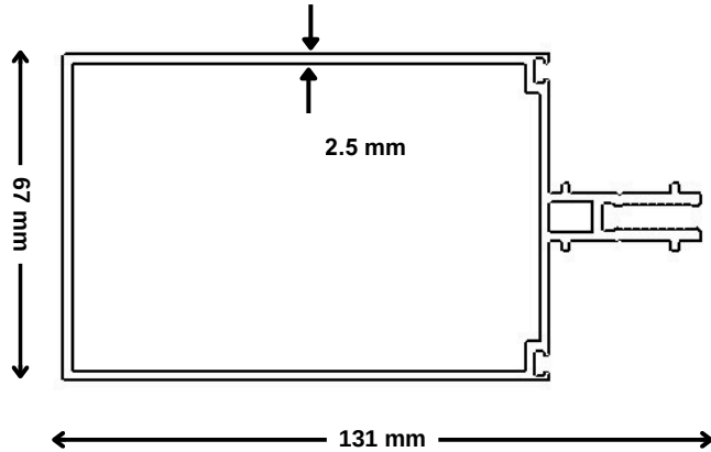
Mullion (101501)
