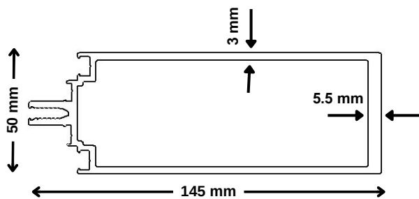
Mullion(101509)
